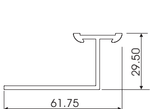
W28002 GLAZING BEADS
